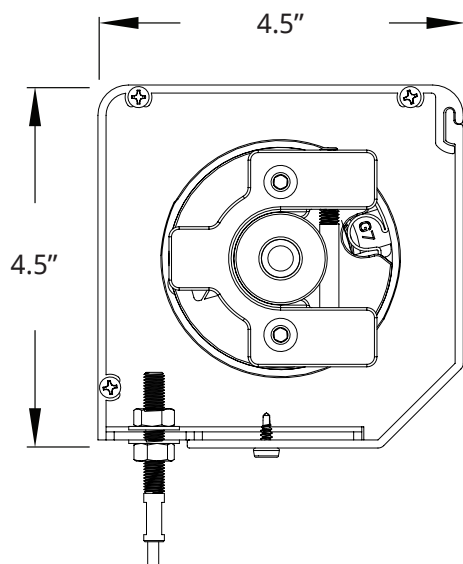
4.5" EXTRUDED ALUMINUM BOX
