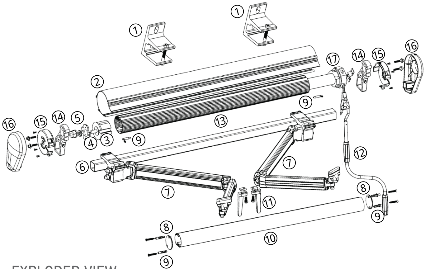
EXPLODED VIEW
