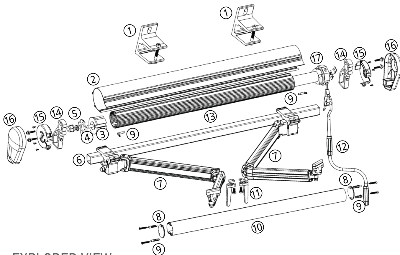
EXPLODED VIEW
