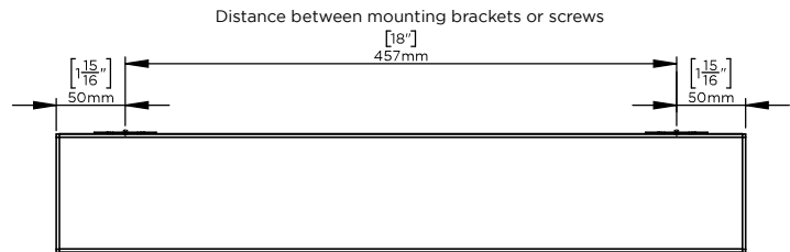
FACE WALL MOUNT
